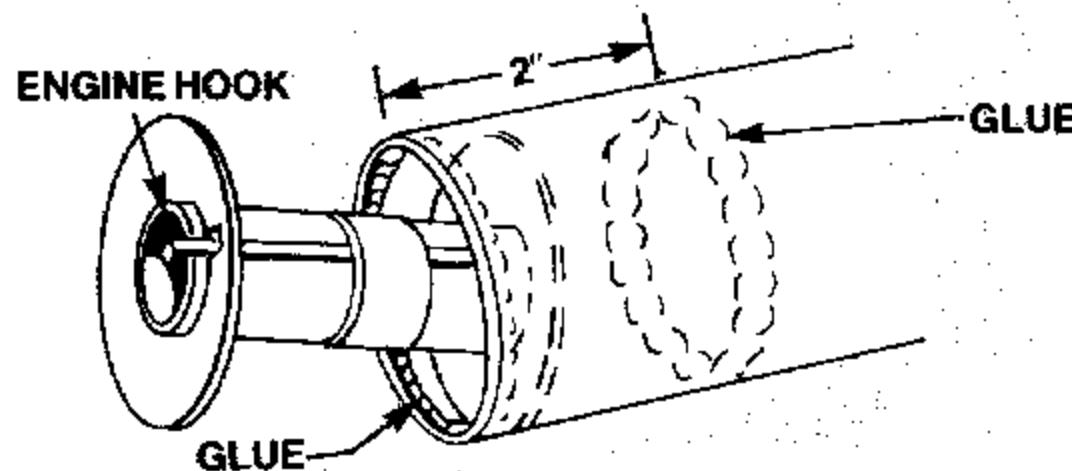
B. INSERT ENGINE MOUNT PART WAY AND APPLY GLUE AROUND REAR OF TUBE
